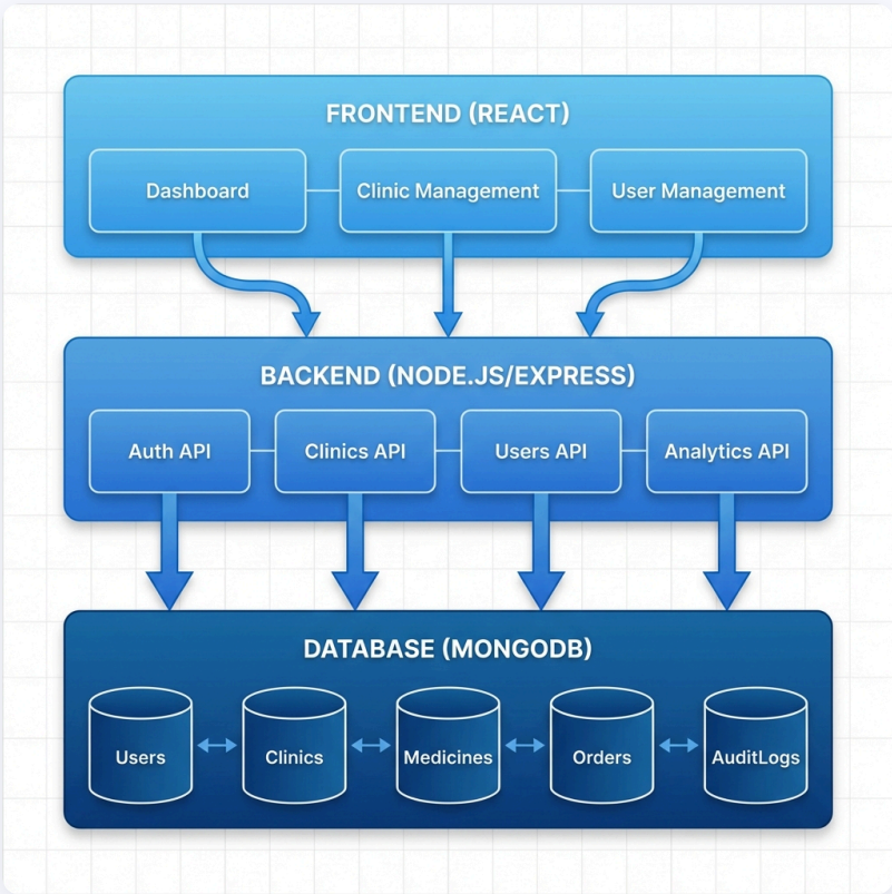
Figure 1: Three-Tier System Architecture
