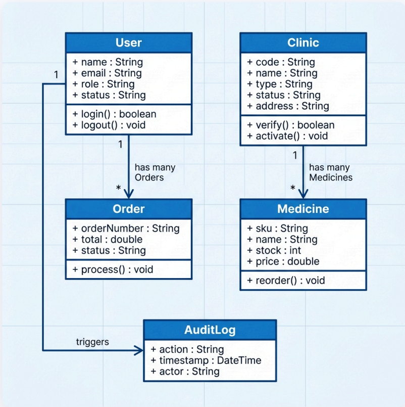
Figure 3: UML Class Diagram - Data Model
