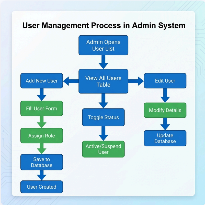
Figure 5: User Management Process Flowchart
