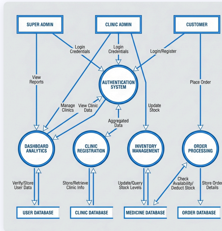
Figure 6: Level-1 Data Flow Diagram
