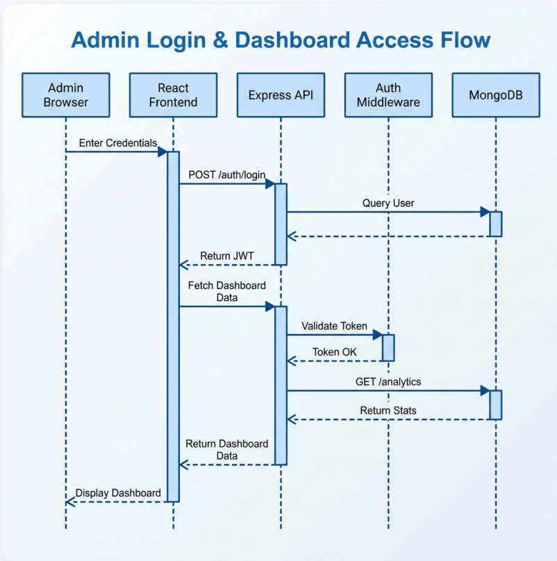
Figure 7: UML Sequence Diagram - Login Flow
