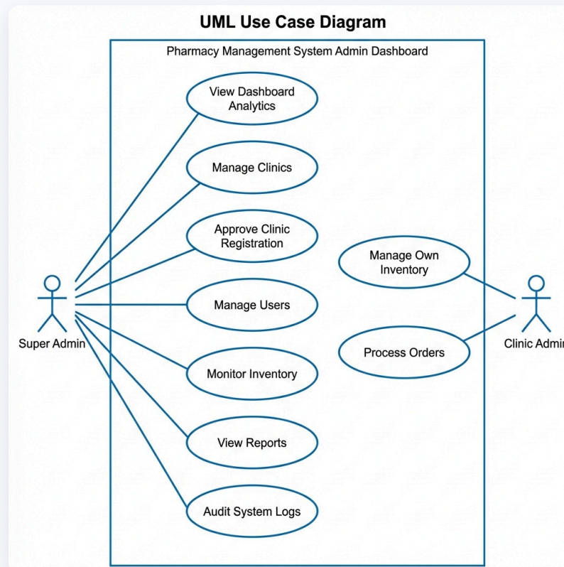
Figure 2: UML Use Case Diagram - Admin Dashboard
