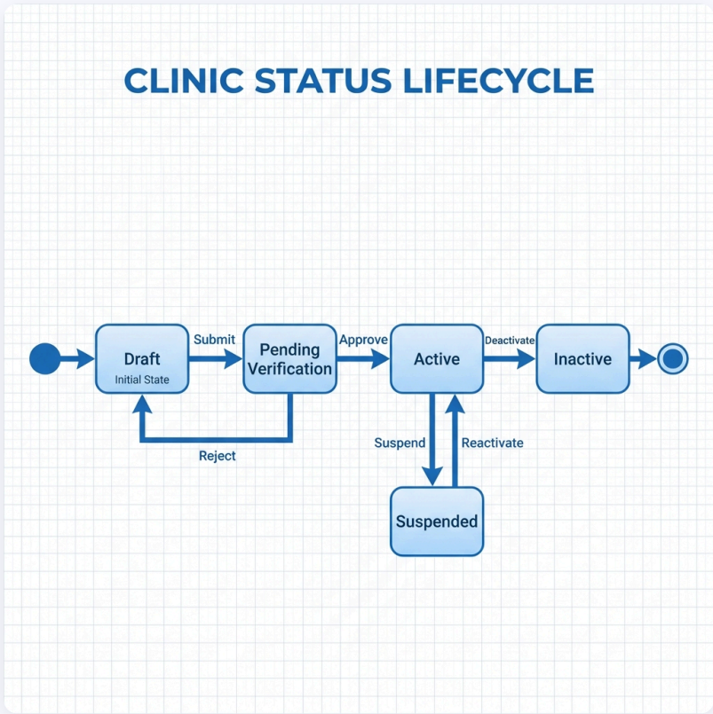
Figure 8: UML State Diagram - Clinic Lifecycle
